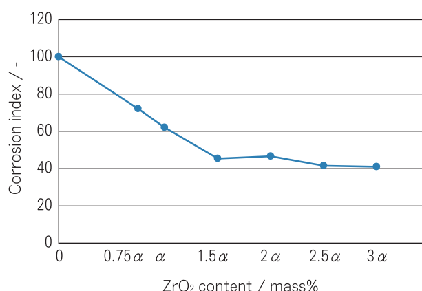
Fig. 4 Index of corrosion by Fe-Co.
