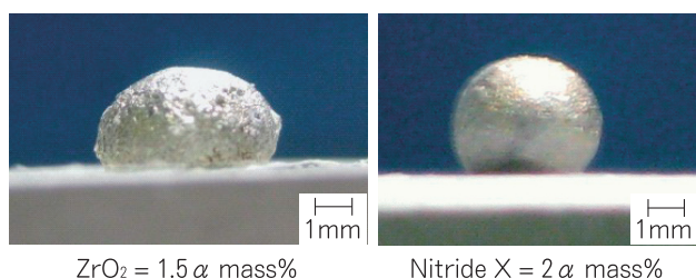
Fig. 7 Metal wetting comparison of \text{ZrO}_2 content 1.5\alpha mass percent product and nitride X content 2\alpha mass percent product.
